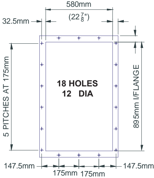
FILTER MAINTAINING FLANGE DETAILS
