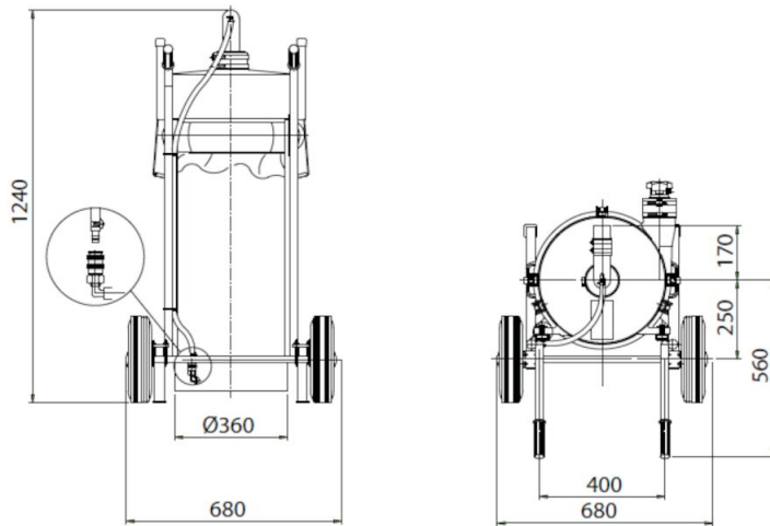
Dimensions FA7 70 liter.
