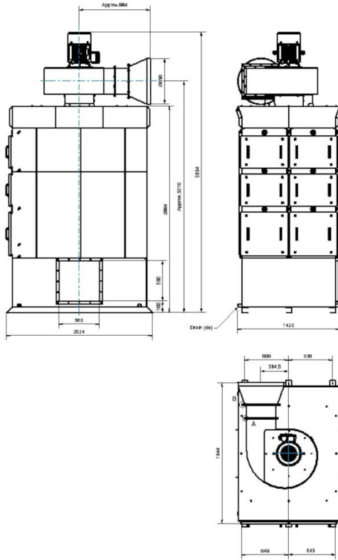
OMF 2x6000 with inlet from right side:
