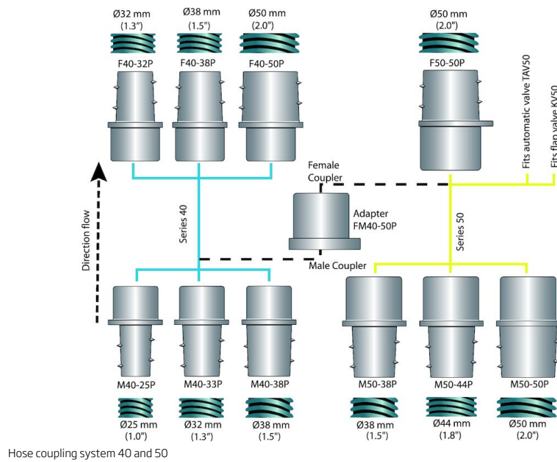
Hose coupling system 40 and 50
