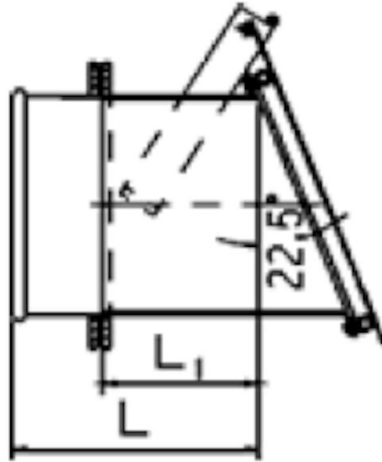
Back pressure flap in vertical wall
